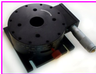
[RSE01]: Rotation Stage, 360° Coarse, 5° Fine Rotation, 0.01° Accuracy, Metric
